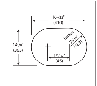
Counter Cutout for Drop-in Dispensers
