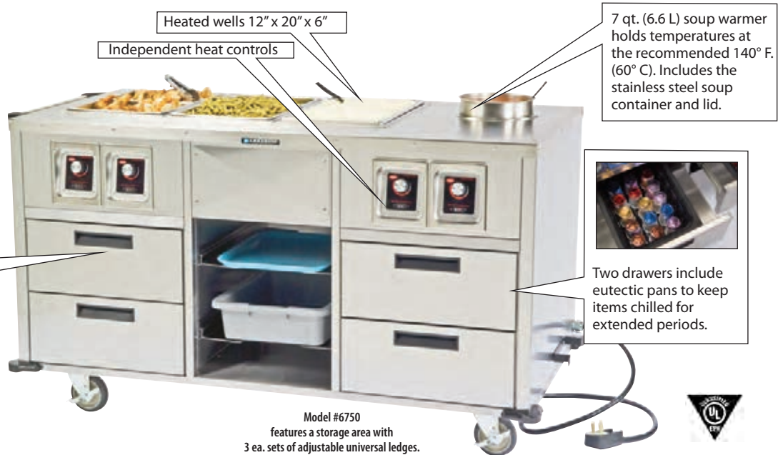
Optional 3 rail tray slide folds down for transport and storage.
